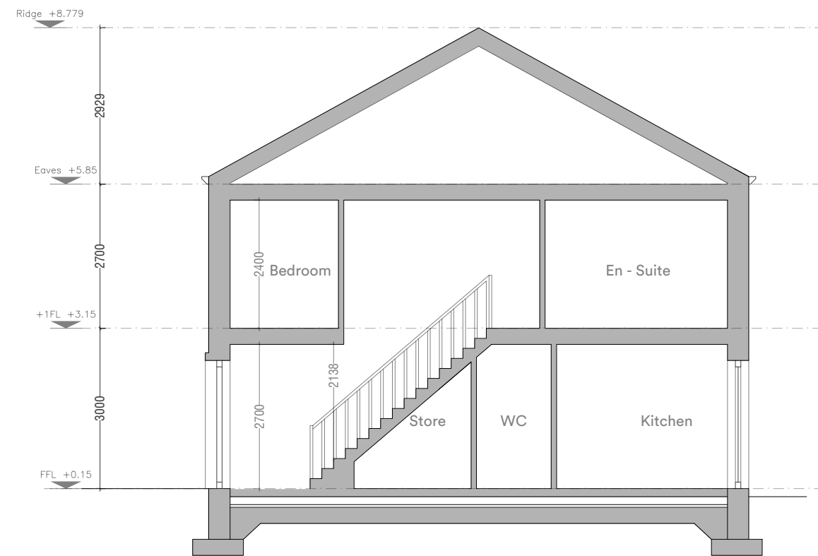
House Type P1 Terraced Section A.A
